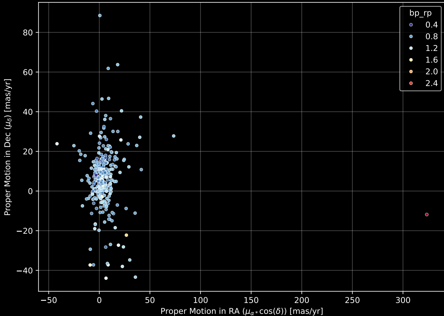
GALAH DR4 Field: [465] Proper Motion Diagram (n= 305)
