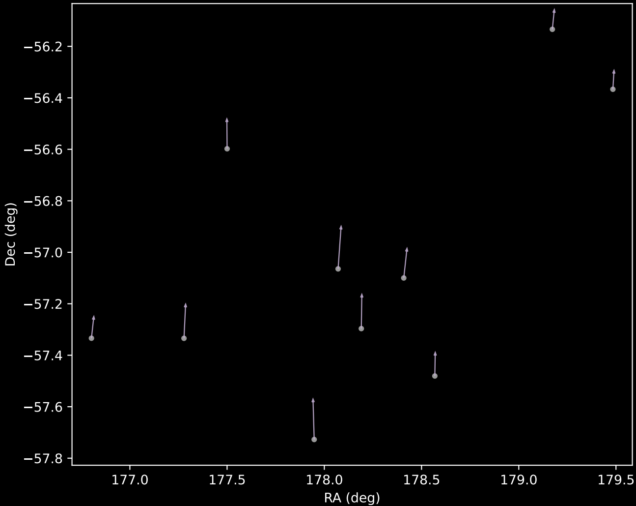
GALAH DR4 Cluster 9 Proper Motion Vectors (n=10)
