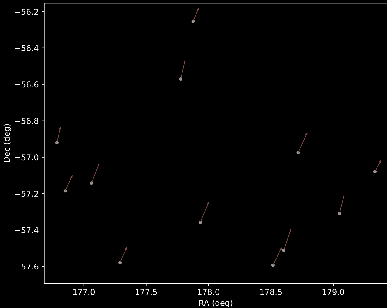
GALAH DR4 Cluster 10 Proper Motion Vectors (n=12)
