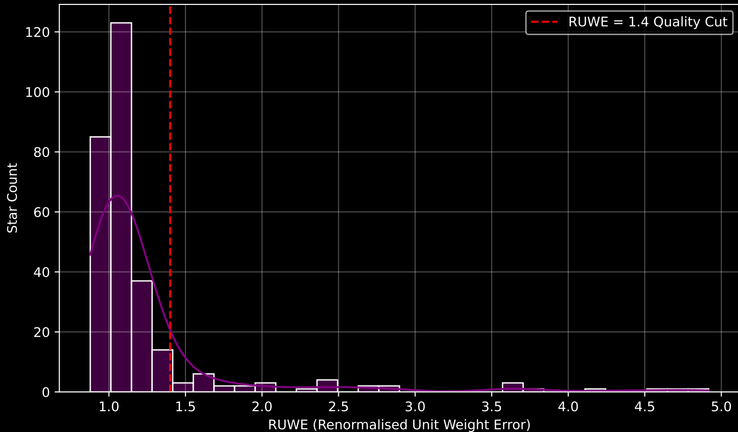
GALAH DR4 Field [465] RUWE Distribution (n= 292)
