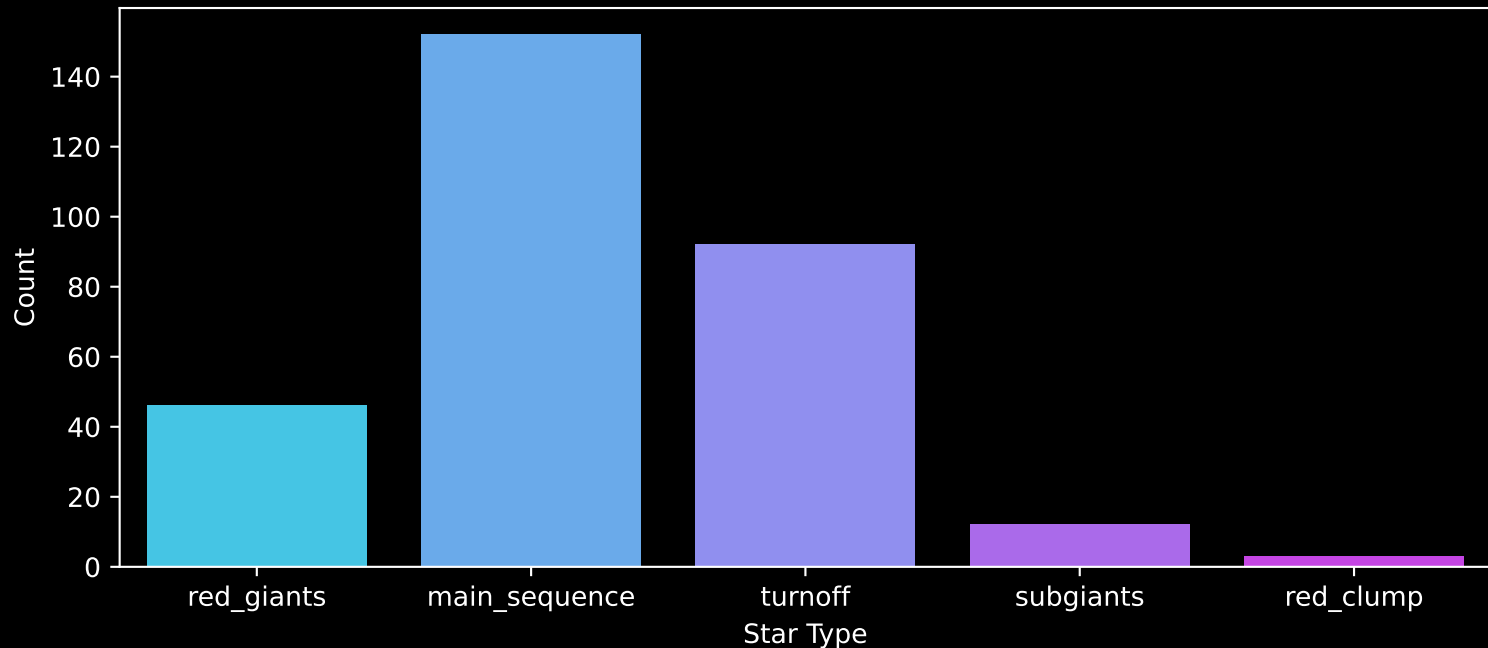
GALAH DR4 Field: [465] Count plot of Star Type
