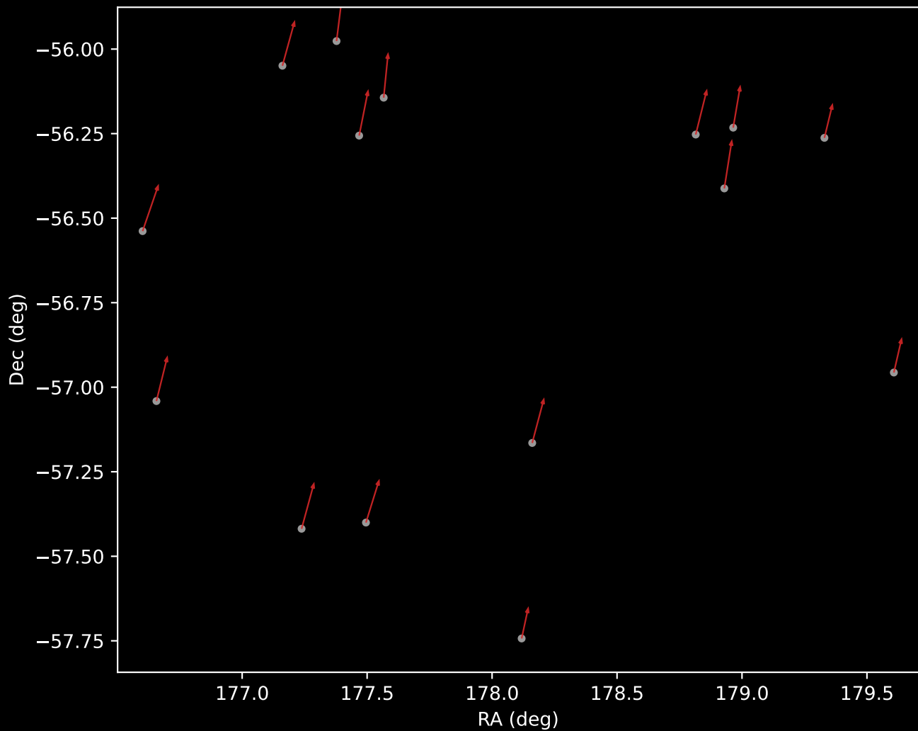
GALAH DR4 Cluster 6 Proper Motion Vectors (n=15)
