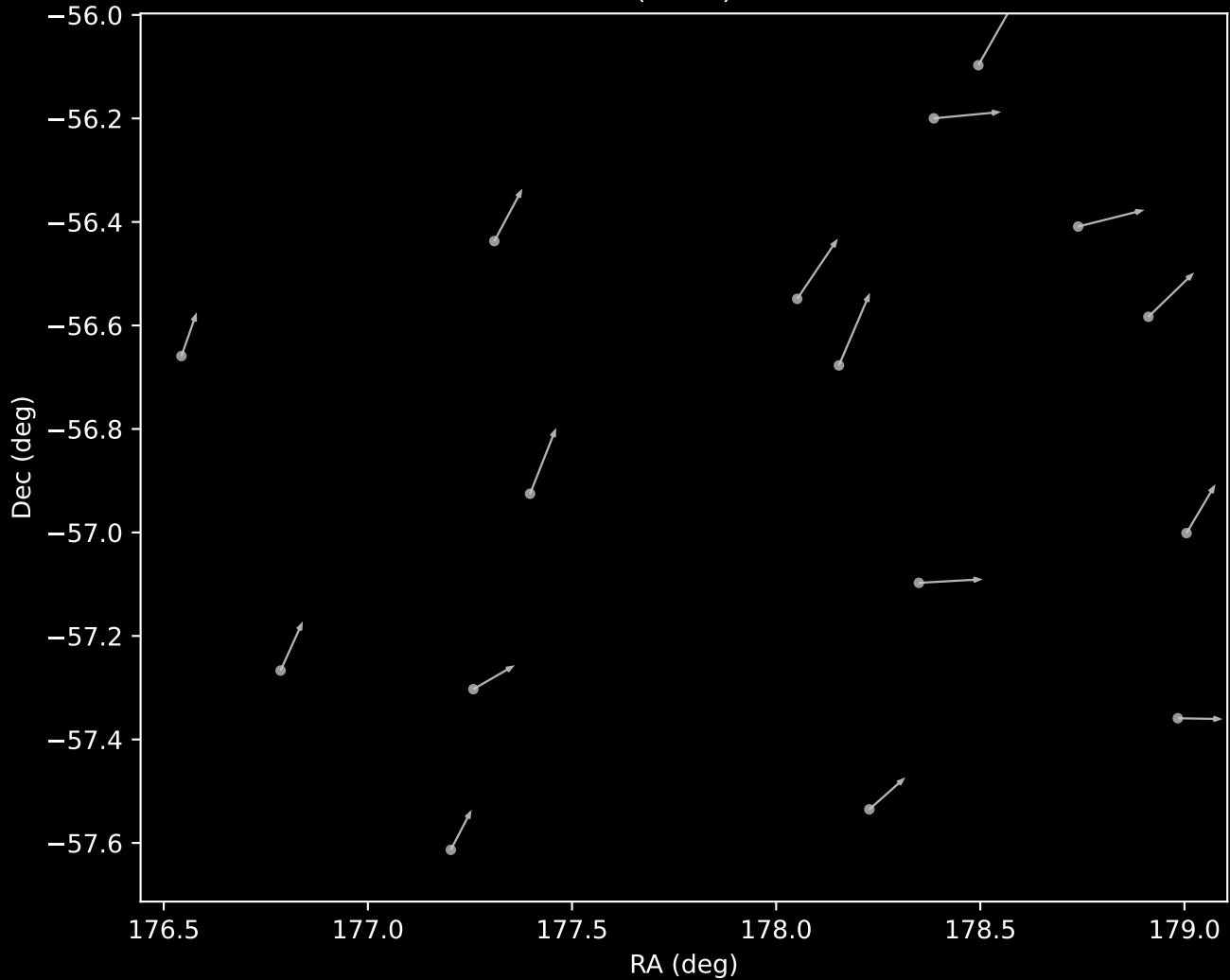
GALAH DR4 Cluster 15 Proper Motion Vectors (n=16)
