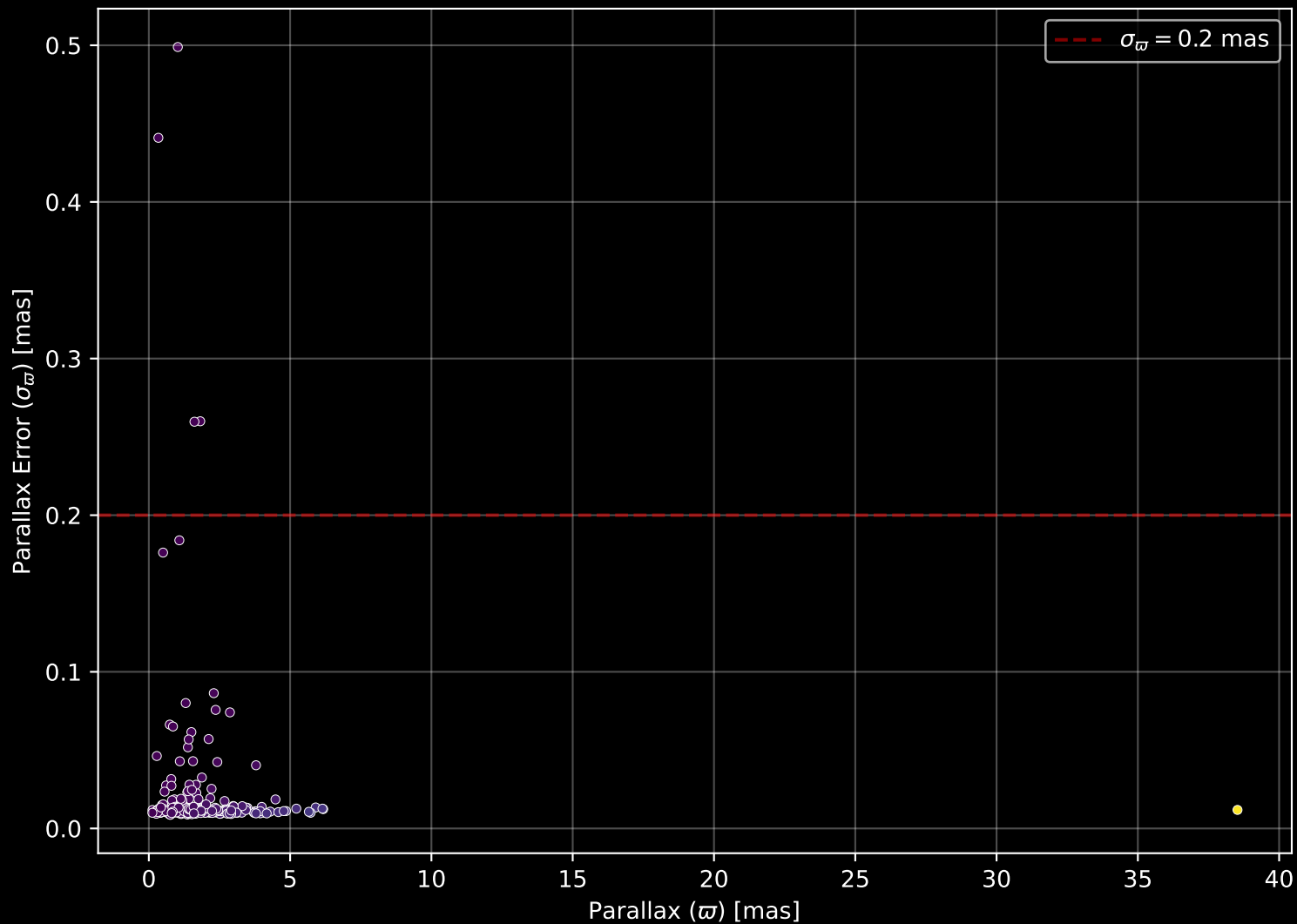
GALAH DR4 Field: [465] Parallax Quality (n= 305)
