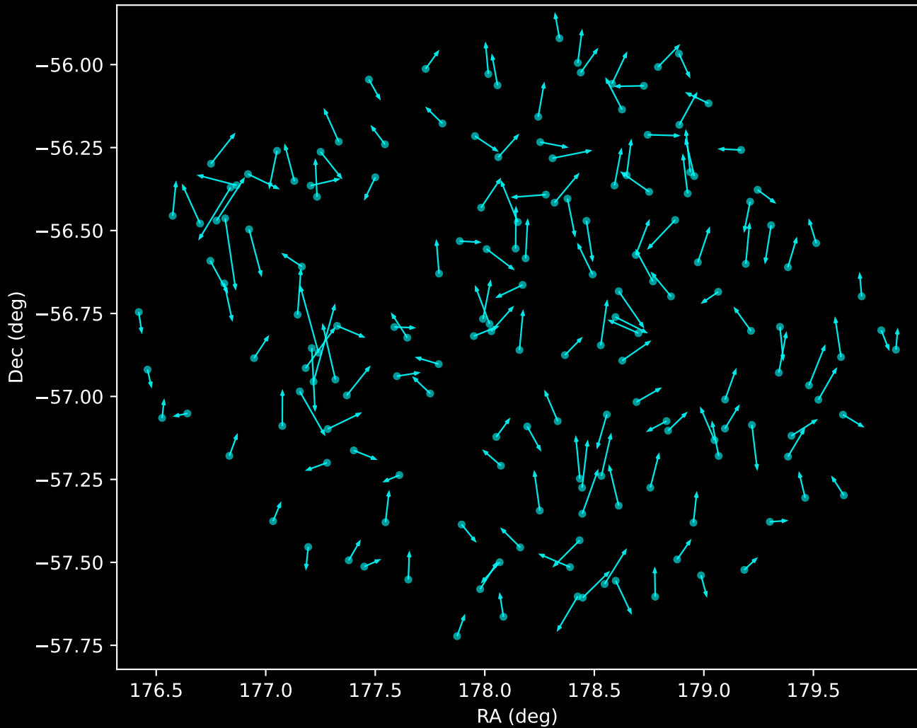
GALAH DR4 Noise Stream Proper Motion Vectors (n=167)
