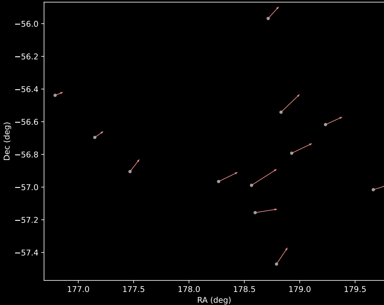
GALAH DR4 Cluster 7 Proper Motion Vectors (n=12)
